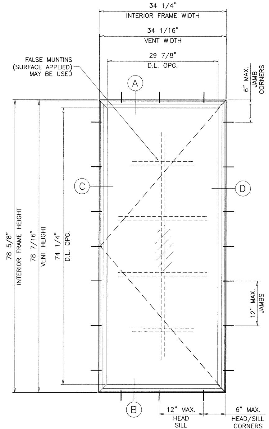
TYPICAL ELEVATION TESTED UNIT
